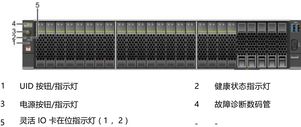
图 3-7 8x2.5 SAS/SATA+12x2.5 NVMe 硬盘配置前面板指示灯和按钮
