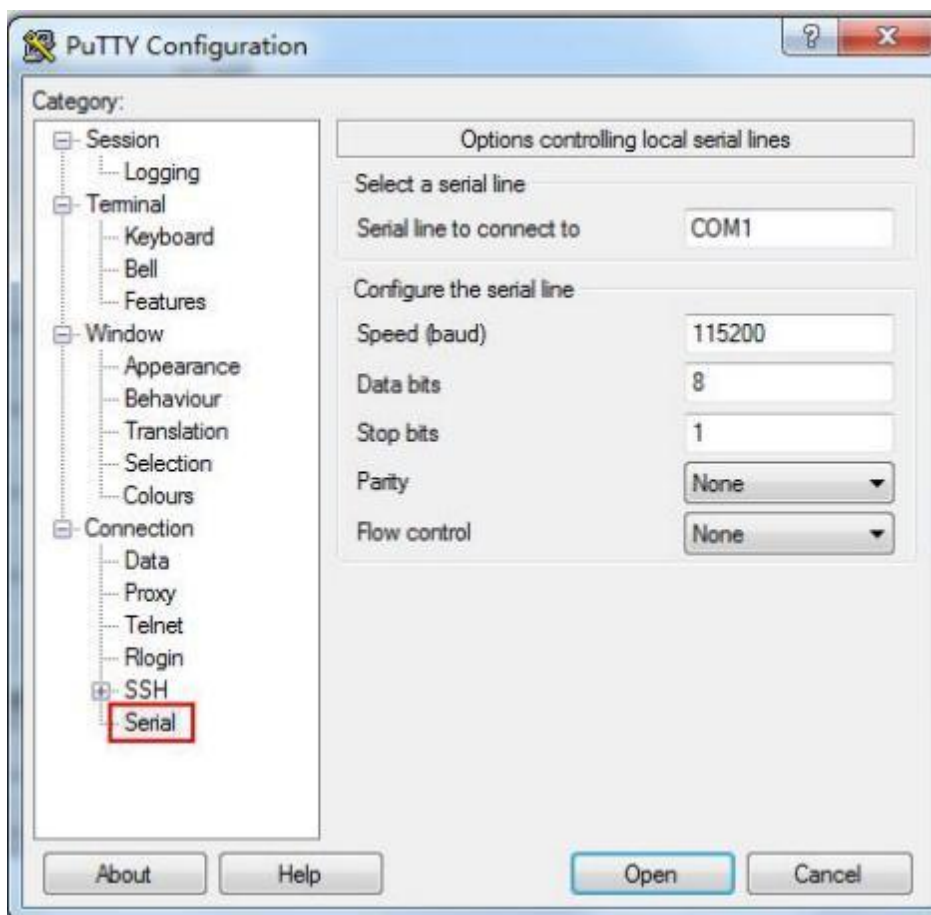
图 8-16 PuTTY Configuration - Serial
